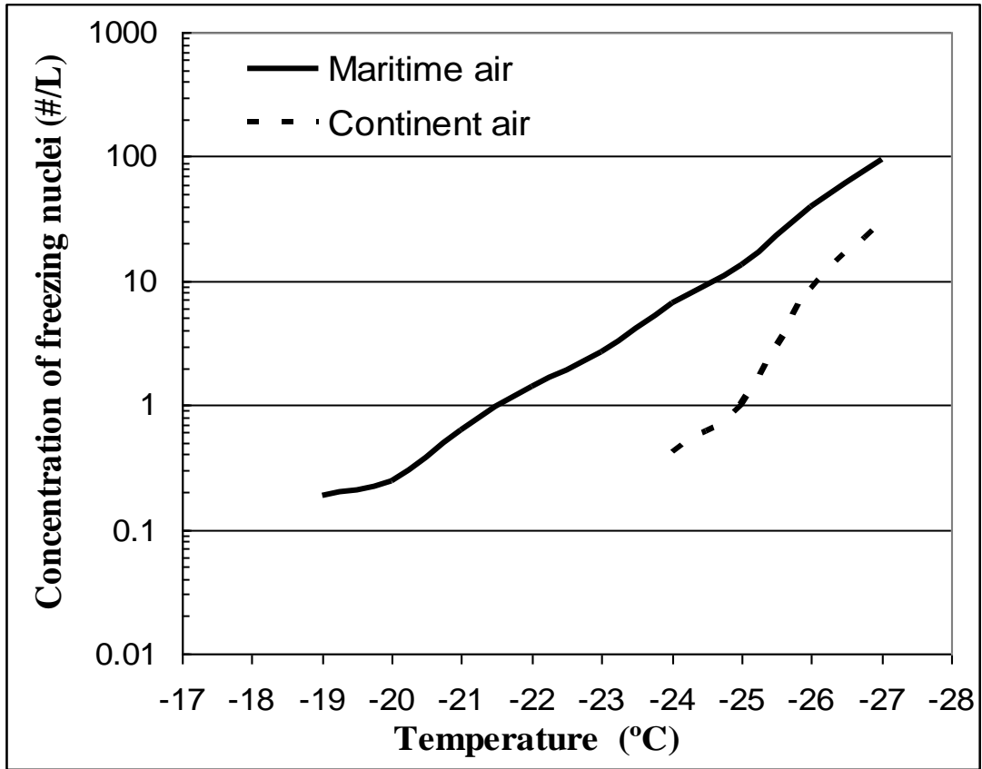
Fig. 9: Comparison between measurements taken on the rooftop based on air trajectory calculations. The solid curve represents ice nuclei concentrations in maritime air mass as measured from filters 1-4 and 8. The dashed curve is for ice nuclei concentrations in continental air mass as measured from filters 9-12. See text for definition of maritime and continental air.
