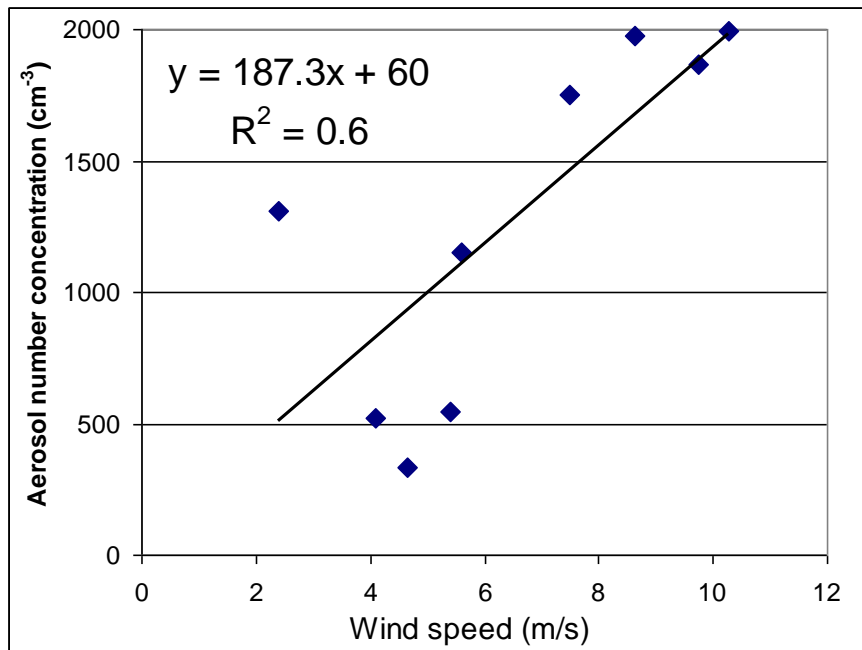
Fig. 7b: Concentration of aerosols > 0.01 μm as a function of wind speed.
