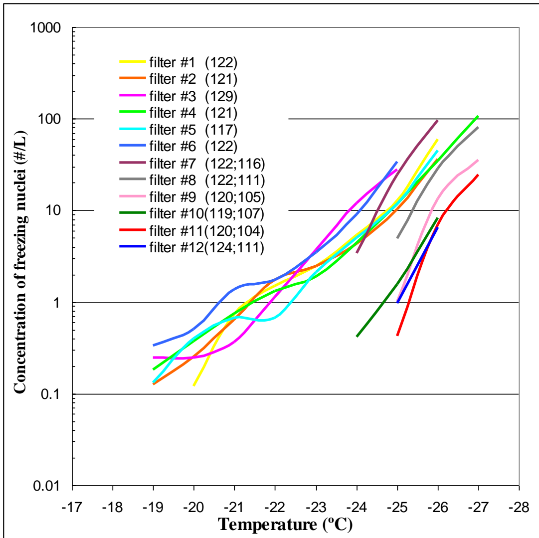
Fig. 4: Concentration of Freezing Nuclei calculated for the different samples. Note that for samples 7-12 all the drops that froze at similar temperatures to the blank filters were removed from the analysis. The first number in the parenthesis represents the number of drops used in the experiment and the second is the one used for the present calculations.
