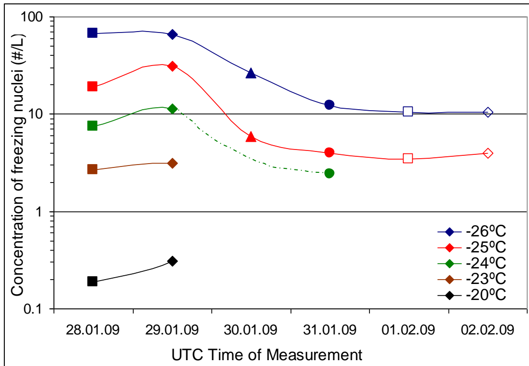
Fig. 6: Concentrations of Freezing Nuclei at different temperatures for the rooftop measurements on different days of the campaign. Each day is represented by a different symbol, and each temperature is represented by a different color.
