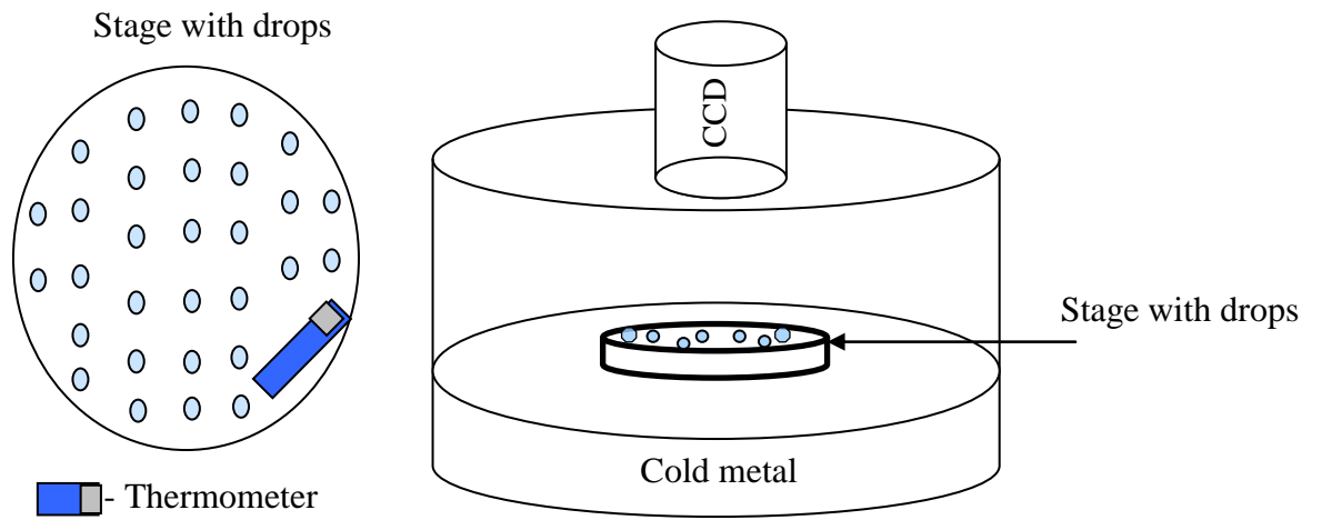
Fig.2: Schematic diagram of the immersion freezing method.
