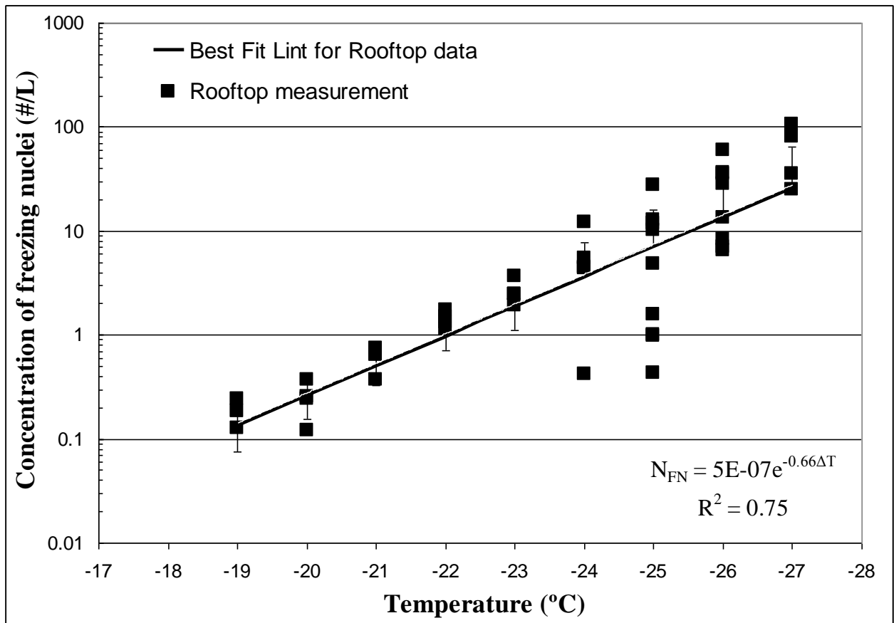
Fig. 10: The concentrations of FN in the air. The equation represents the best fit line to the rooftop data.
