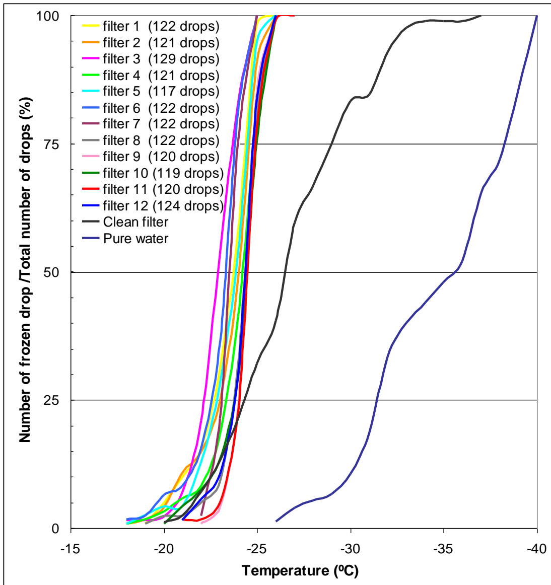
Fig. 3: The cumulative freezing spectrum of all the South Pole samples and the average spectrum of freezing temperature from clean filters and pure water.
