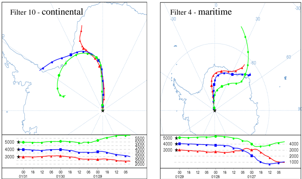
Fig. 8: Two examples of back trajectories of continental air collected on filter 10 and maritime air that was sampled on filter 4. The maps show the trajectory that the air parcels travel before reaching the station, located at an altitude of about 3000m ASL. The vertical projection for air arriving from 3000, 4000 and 5000 m is shown. Source: http://www.arl.noaa.gov .
