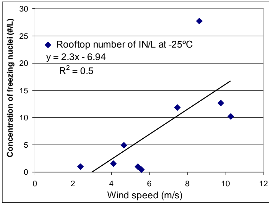
Fig. 7a: Concentration of freezing nuclei at -25°C as a function of wind speed.
