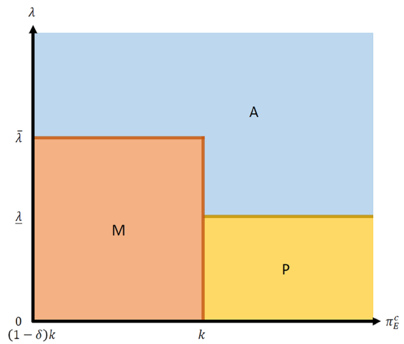
FIGURE 2 | Equilibrium selection.
