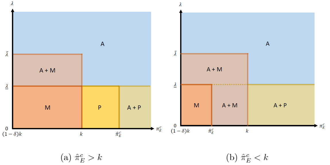
Figure 1: Equilibrium outcomes
