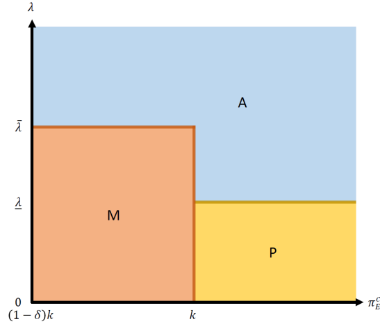
Figure 2: Equilibrium selection
