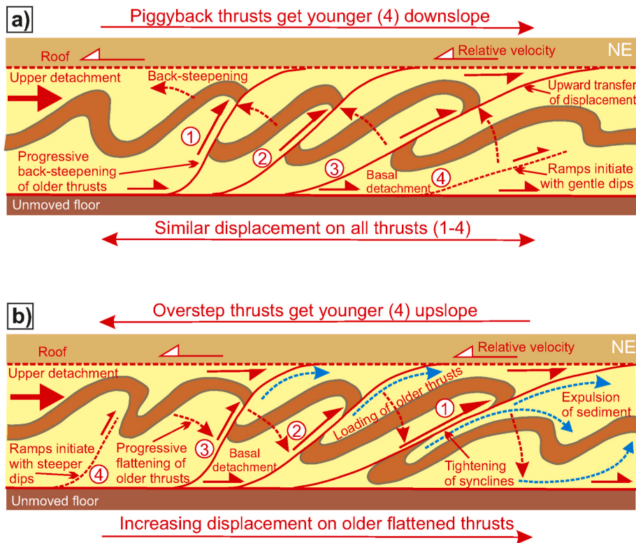
Fig. 12. Summary cartoon showing a) downslope-propagating piggyback thrust sequences, and; b) upslope-propagating overstep thrust sequences. In piggyback thrusting (a), new gently-dipping thrusts (4) develop in the footwalls of existing thrusts thereby causing a rotation and progressive back-steepening of the older, overlying thrusts. In overstep thrusting (b), new moderately-dipping thrusts (4) form in the hangingwalls of existing thrusts and progressively load and flatten the underlying pinched synclines resulting in reduced dips of underlying thrusts. Continued movement on thrusts during loading results in greater displacement on gently-dipping thrusts.
