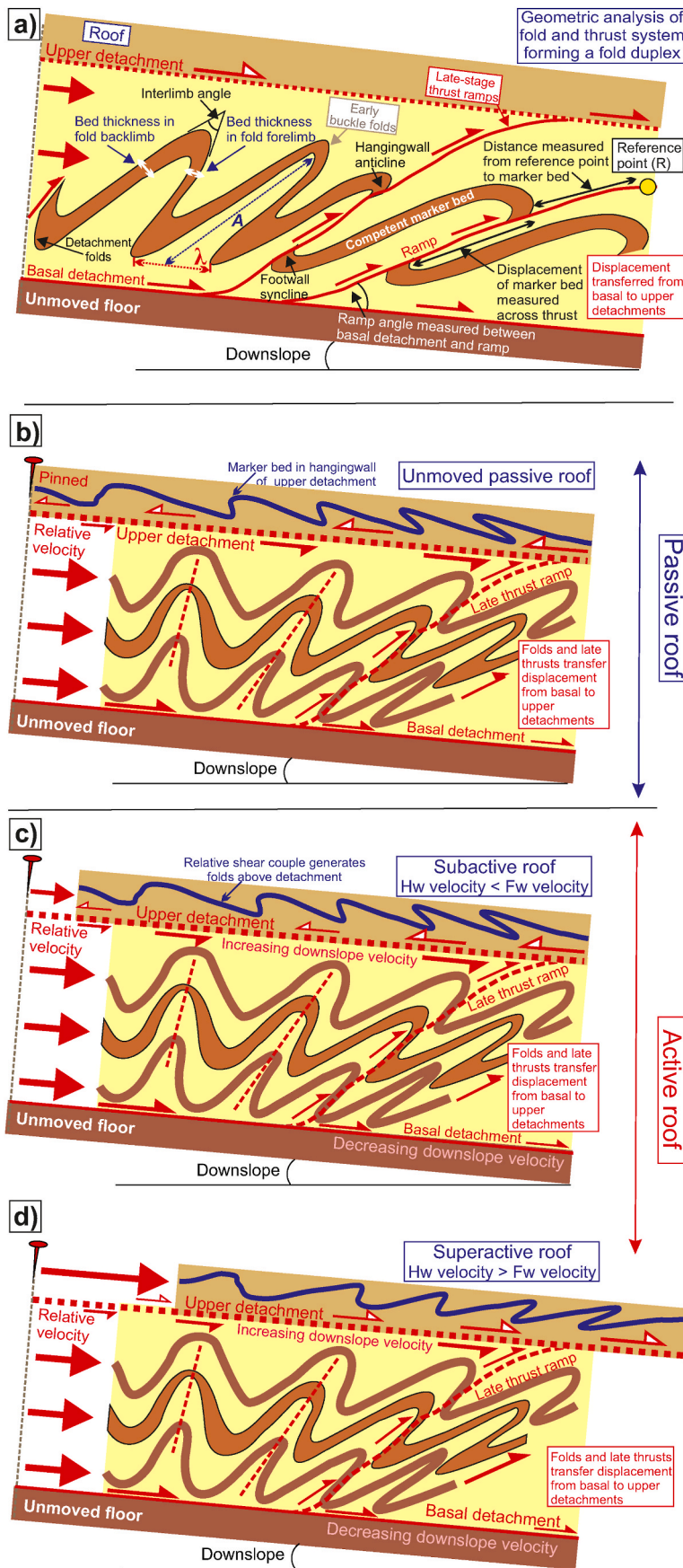
Fig. 1. a) Schematic cartoon of a fold duplex that illustrates geometric parameters such as bed thicknesses, ramp angles, fold wavelengths ( \lambda ) and amplitude ( A ) that are measured around early buckle folds and late thrusts within the fold and thrust system (FATS). b) Schematic cartoon illustrating how the roof above the upper detachment may be passive and remains fixed and unmoved (pinned) relative to the sequence beneath the basal detachment. Differences in relative downslope velocity between the roof and underlying FATS generate a shear couple that creates upslope-verging folds in the hangingwall of the upper detachment. c) Schematic cartoon illustrating how the roof above the upper detachment may be active and moves downslope more slowly than the underlying FATS. The roof is sub-active with the hangingwall velocity ( Hw\ V ) above the upper detachment being less than the footwall velocity ( Fw\ V ) beneath it ( Hw\ V < Fw\ V ). This difference in relative downslope velocity generates a shear couple that creates upslope-verging folds in the hangingwall of the upper detachment. d) Schematic cartoon illustrating how the roof above the upper detachment may be active and moves downslope more rapidly than the underlying FATS. The roof is super-active with the hangingwall velocity above the upper detachment being greater than the footwall velocity beneath it ( Hw\ V > Fw\ V ). This difference in relative downslope velocity generates a shear couple that creates downslope-verging folds in the hangingwall of the upper detachment. In all cases, the folds and late thrusts are considered to transfer displacement from the basal to upper detachments to create a fold duplex.
