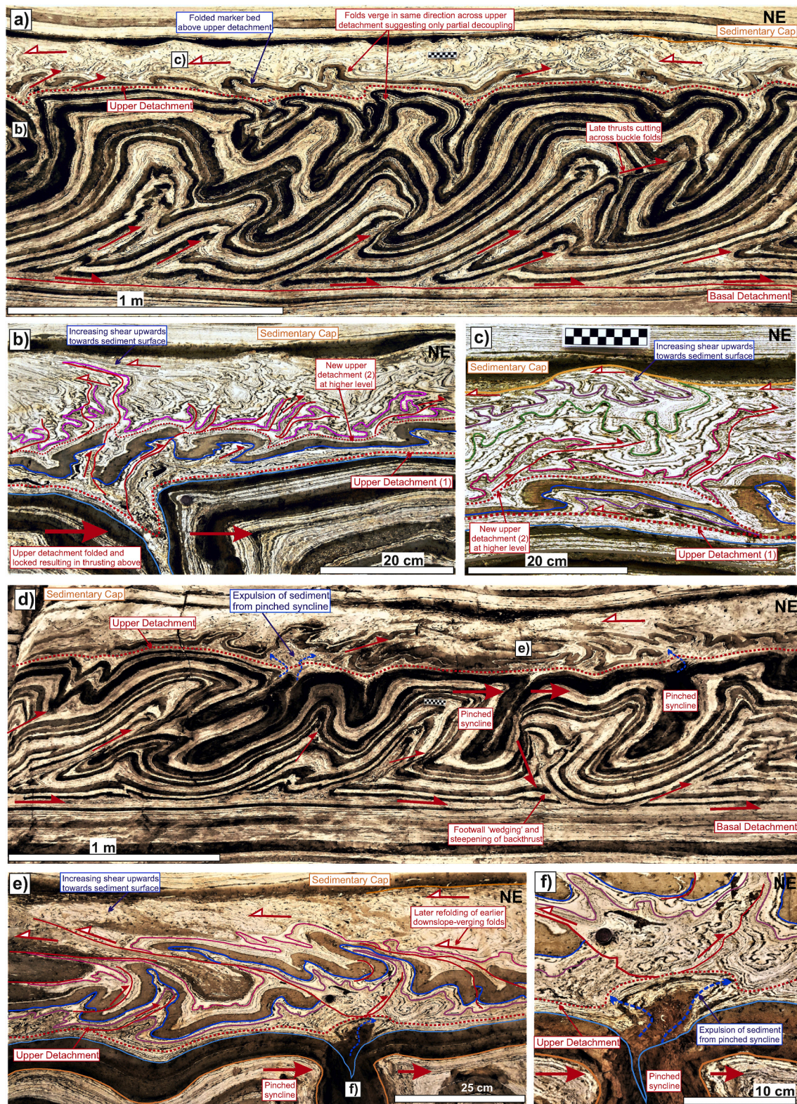
Fig. 8. Detailed photographs of pinched synclines and upper detachment in the studied section (see Fig. 3e for locations). Photograph a) shows that in some instances folds verge in the same direction above and below the upper detachment (red dotted line), thereby suggesting only partial decoupling across this structure. Photographs b, c) and e, f) show further details of the upper detachment in each case. b) Pinching shut of synclines causes local folding and imbrication of the blue marker layer above the upper detachment, together with the development of new higher-level detachments (2). E) Refolding of folds in the blue marker layer with increasing shear upwards towards the sediment surface. Scale is provided by the 10 cm chequered rule and 15 mm diameter coin. (For interpretation of the references to colour in this figure legend, the reader is referred to the Web version of this article.)
