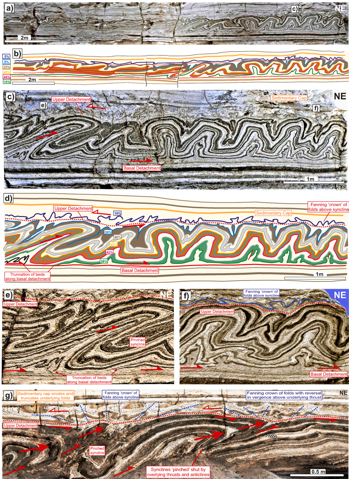
Fig. 9. a, c) Photographs and b, d) associated line drawings of the FATS (see Fig. 2e for location). The amount of % shortening across different marker layers is shown in the boxes in b) and d). Photograph e) shows details (from c) of stratigraphic cut-offs along the basal detachment, while f) shows fanning folds above the upper detachment (red dotted line). f) Fanning crowns of folds formed above the upper detachment and underlying thrusts and synclines. Note that fanning folds are truncated by the overlying sedimentary cap. Scale is provided by the 10 cm chequered rule. (For interpretation of the references to colour in this figure legend, the reader is referred to the Web version of this article.)
