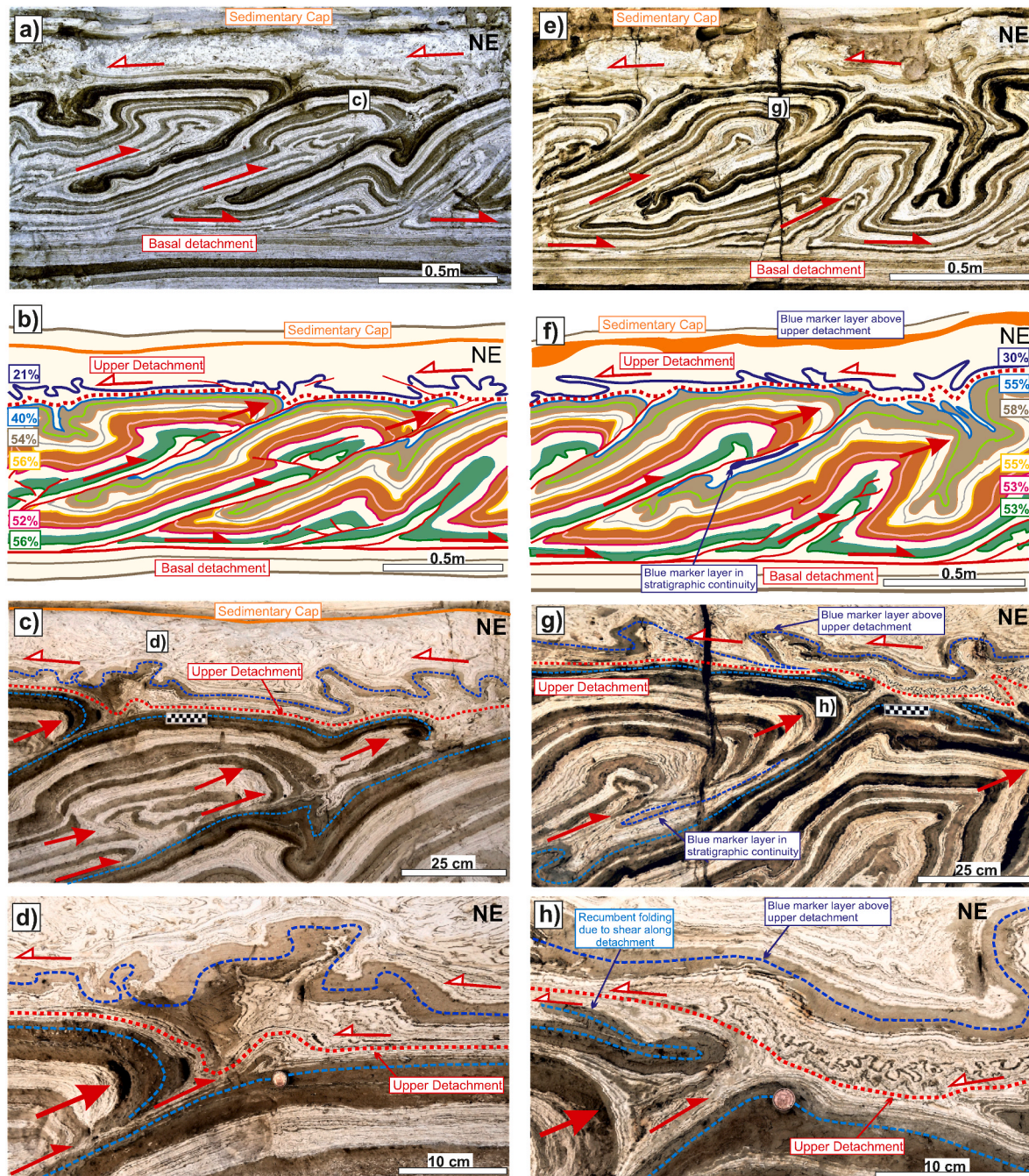
Fig. 7. a, e) Photographs and b, f) associated line drawings of the FATS (see Fig. 3b, g for locations, and Fig. 5a, e for further data). The amount of % shortening across different marker layers is shown in the boxes. Photographs c, d) and g, h) show details of the upper detachment (red dotted line) in each case. Large displacements along thrust ramps are transferred onto the upper detachment leaving the overlying blue marker horizon unaffected by thrusts and with SW-verging folds. The blue marker layer is also locally trapped in synclinal cores (g) beneath the upper detachment. Scale is provided by the 10 cm chequered rule and 15 mm diameter coin. (For interpretation of the references to colour in this figure legend, the reader is referred to the Web version of this article.)
