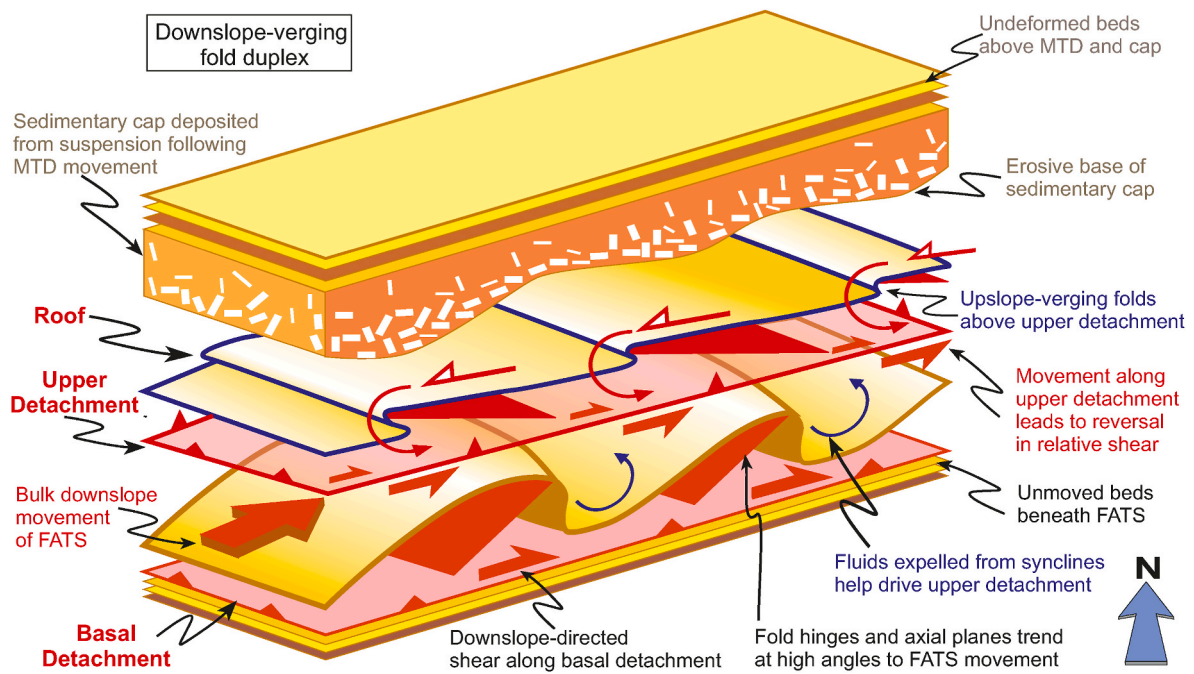
Fig. 15. Summary cartoon of reversals in relative shear sense across upper detachments that bound fold duplexes in gravity-driven FATS. Folds formed in the hangingwall of the upper detachment are typically coaxial to, but verge in the opposite sense to folds in the underlying downslope-translating FATS. The overlying sedimentary cap is deposited out of suspension following cessation of movement that creates the MTD and may in some cases erode the upper detachment.
