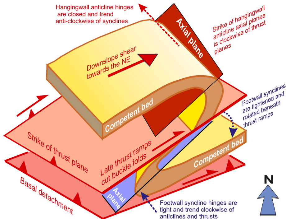
Fig. 13. Summary cartoon based on orientation data in Fig. 6, highlighting geometric obliquities between hangingwall anticlines and adjacent footwall synclines developed across late thrust ramps. Synclines are generally tighter, and trend clockwise of anticlines, due to loading from overlying thrust ramps and progressive shear during continued downslope translation. See text for further discussion.
