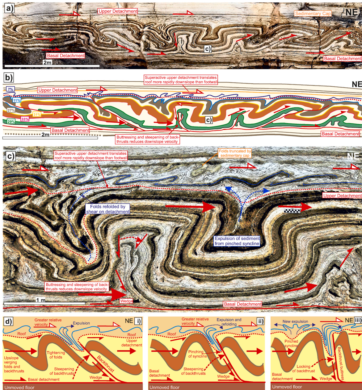
Fig. 11. a) Photograph and b) associated line drawing of backthrust system (see Fig. 2e for location). The amount of % shortening across different marker layers is shown in the boxes in b). Photograph c) show details of backthrusting, together with folding of the blue marker layer above multiple upper detachments (red and pink dotted lines). Scale is provided by the 10 cm chequered rule. d) Schematic summary cartoons illustrating the role of fold tightening in generating a range of potential fold and thrust geometries. Structures are shown evolving from an early stage (i) to a later stage (iii) during downslope translation of FATS. Backthrust ramps are progressively steepened resulting in earlier buckle folds being systematically tightened and synclines 'pinched' during expulsion of sediments from fold cores. Reversals in fold vergence in the blue marker bed reflect variations in relative downslope velocity across the upper detachment, with fanning crowns of folds formed above tightened synclines. (For interpretation of the references to colour in this figure legend, the reader is referred to the Web version of this article.)
