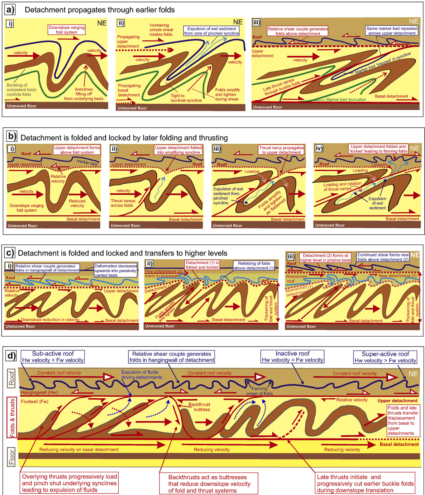
Fig. 14. Schematic summary cartoons highlighting the role of variations in relative velocity across upper detachments in generating a range of potential fold and thrust geometries. In each case, structures are shown evolving from an early stage (i) to a later stage (iii) during progressive downslope translation of FATS. a) A relatively late-stage upper detachment propagates across and truncates earlier buckle folds that are systematically tightened and ‘pinched’ during expulsion of sediments from fold cores. b) Upper detachment is folded by continued shortening in FATS resulting in a fanning ‘crown’ of folds above the ‘locked’ detachment. c) Upper detachment is folded and ‘locked’ by continued shortening in FATS, resulting in displacement transferring to a higher level to create a new upper detachment (2). d) Synthesis cartoon illustrating how variations in relative hangingwall velocity (Hw) and footwall velocity (Fw) across the upper detachment create sub-active roofs, inactive roofs and super-active roofs. Displacement is transferred from the basal detachment to the upper detachment via folds and late-stage thrusts.
