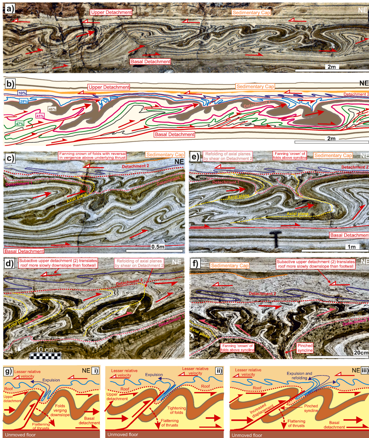
Fig. 10. a) Photograph and b) associated line drawing of the FATS (see Fig. 2e for location). The amount of % shortening across different marker layers is shown in the boxes in b). Photographs c, d) and e, f) show details of folding above multiple upper detachments (red and pink dotted lines), together with refolding of earlier axial planes. Scale is provided by the 10 cm chequered rule. g) Schematic summary cartoons illustrating the role of fold tightening in generating a range of potential fold and thrust geometries. Structures are shown evolving from an early stage (i) to a later stage (iii) during downslope translation of FATS. Thrust ramps are progressively flattened resulting in earlier buckle folds being systematically tightened and ‘pinched’ during expulsion of sediments from fold cores. Reversals in fold vergence in the blue marker bed reflect variations in relative downslope velocity across the upper detachment (see Fig. 1b–d). (For interpretation of the references to colour in this figure legend, the reader is referred to the Web version of this article.)
