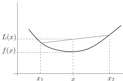
FIGURE 17. Convexity
