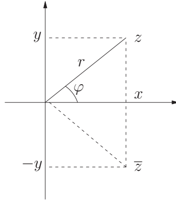
FIGURE 19. Complex plane
