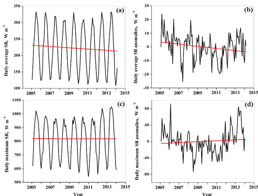
Figure 4. Monthly variations of (a, b) daily average surface solar radiation (SR); and (c, d) daily maximum surface solar radiation, based on pyranometer measurements at the hydrometeorological buoy anchored in the Dead Sea. The left column represents original monthly data, while the right column represents their associated deseasonalized monthly anomalies. The red straight lines designate linear fits.
