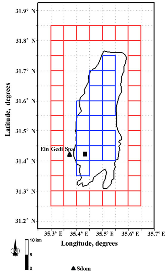
Figure 1. Map of the region under study. The 17 blue boxes show pixels covering the Dead Sea surface. The 34 red boxes show pixels which cover the land area in the vicinity of the Dead Sea. The black square shows the location of the Dead Sea hydrometeorological buoy ( 31.42^\circ \text{ N} , 35.44^\circ \text{ E} ), while the black triangles show the location of two meteorological stations: Sdom ( 31.03^\circ \text{ N} , 35.39^\circ \text{ E} ) and Ein Gedi Spa ( 31.42^\circ \text{ N} ; 35.38^\circ \text{ E} ).
