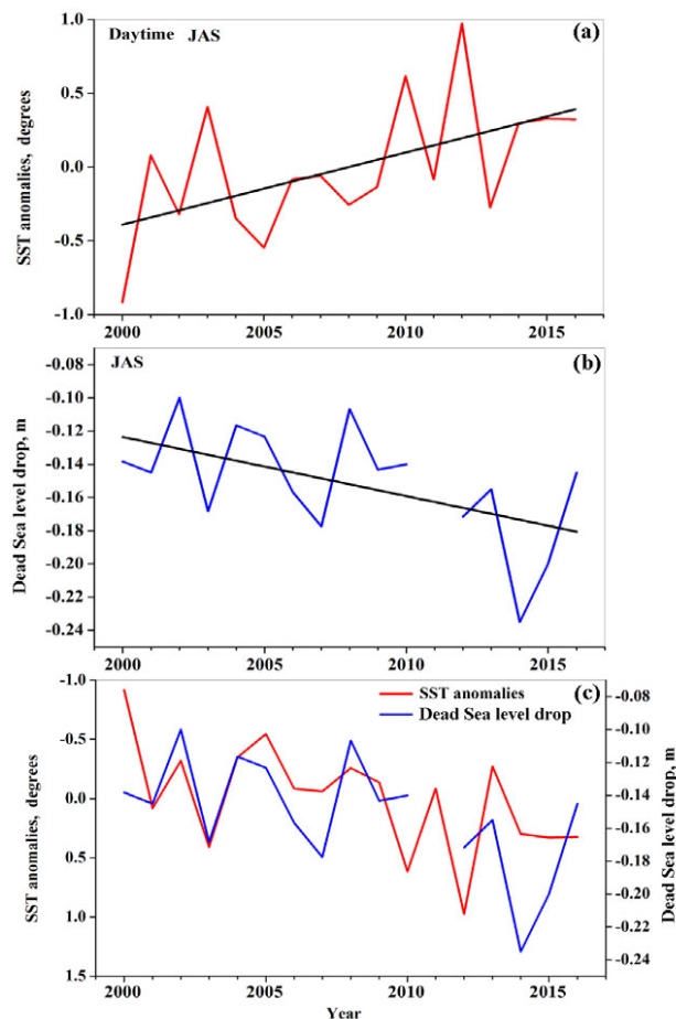
Figure 10. Year-to-year variations in (a) daytime SST anomalies and (b) Dead Sea water-level drop, averaged over the three summer months July, August and September (JAS) characterized by the largest Dead Sea water-level drop. Panel (c) is a comparison between the temporal variations in daytime SST anomalies and Dead Sea water-level drop averaged over the same three summer months. For illustrative purposes, the decreasing scale of SST anomalies is used in panel (c) instead of the increasing scale used in panel (a). One can see that these variations are correlated representing an inverse relationship.
