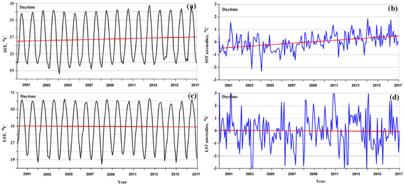
Figure 2. Daytime monthly variations of (a, b) Dead Sea surface temperature (SST) together with (c, d) land skin temperature (LST) over the land area in the vicinity of the Dead Sea, during the 17-year period under study. The left column represents original MOD11C3 Level 3 monthly data (averaged over the specified sea and land areas), while the right column represents their associated deseasonalized monthly anomalies. The red straight lines designate linear fits.
