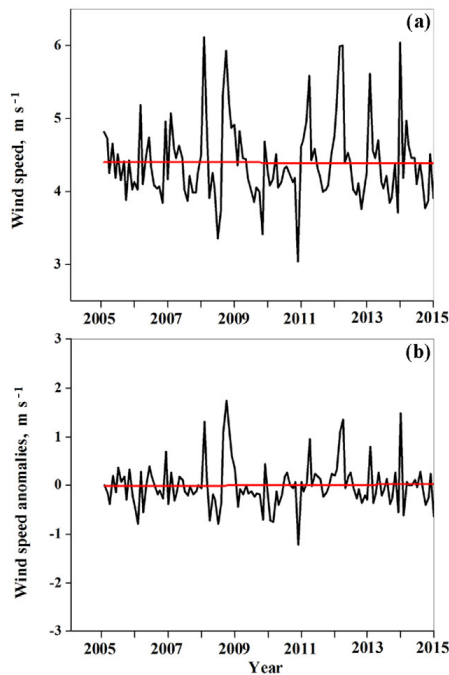
Figure 5. Monthly variations of daily average near-surface wind speed based on wind measurements at the hydrometeorological buoy anchored in the Dead Sea: panel (a) represents original monthly data, while panel (b) represents their associated deseasonalized monthly anomalies. The red straight lines designate linear fits.
