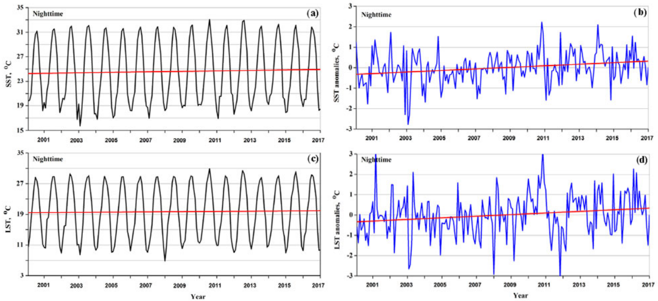
Figure 3. Nighttime monthly variations of (a, b) Dead Sea surface temperature (SST) together with (c, d) land skin temperature (LST) over the land area in the vicinity of the Dead Sea, during the 17-year period under study. The designations are the same as in Fig. 2.
