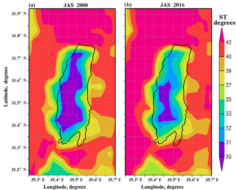
Figure 12. Comparison of the spatial distribution of daytime surface temperature (ST, °C) over the Dead Sea and surrounding land areas (averaged over the JAS summer months) between the years of 2000 and 2016.
