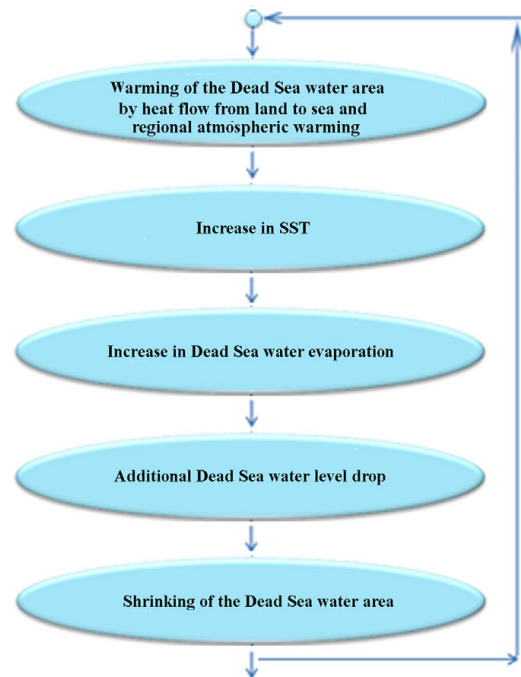
Figure 8. The flowchart of a positive feedback loop between positive Dead Sea surface temperature trends and Dead Sea shrinking.
