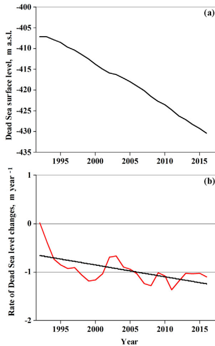
Figure 7. (a) Yearly data of the Dead Sea levels (based on available measurements from 1992 to 2016); (b) the rate of Dead Sea level changes from year to year. The black straight line designates the linear fit.
