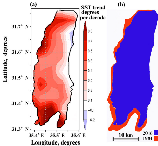
Figure 13. (a) Spatial distribution of 17-year trends of daytime Dead Sea SST ( ^{\circ}\text{C decade}^{-1} ) averaged over the JAS summer months: July, August and September. (b) The Dead Sea water area in the 2 years: 1984 and 2016, based on data from the Google Earth Engine (Gorelick et al., 2017).
