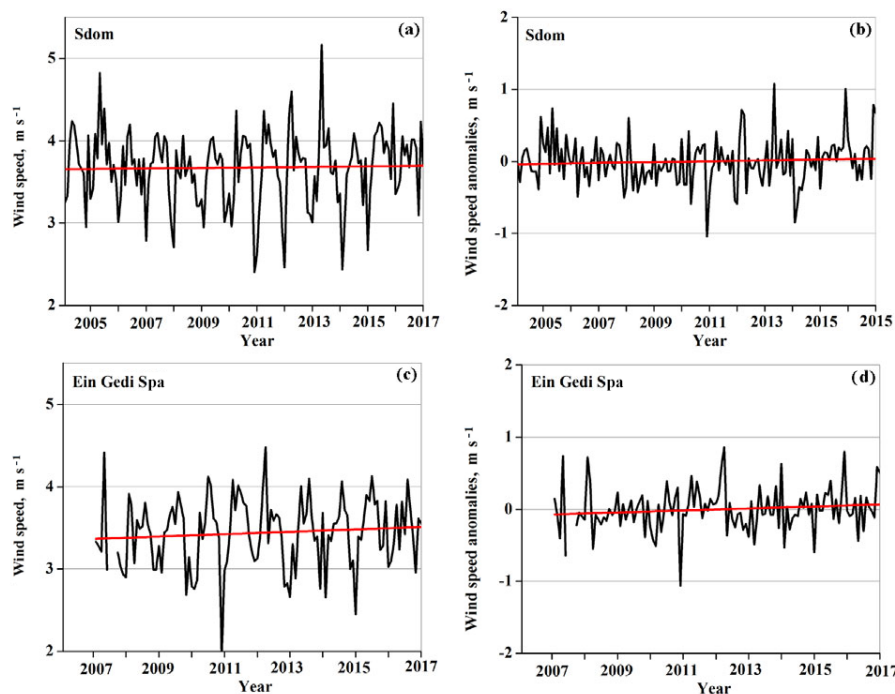
Figure 6. Monthly variations of daily average near-surface wind speed based on wind measurements at two meteorological stations, located in the vicinity of the Dead Sea: (a, b) Sdom (31.03° N, 35.39° E) and (c, d) Ein Gedi Spa (31.42° N; 35.38° E). The left column represents original monthly data, while the right column represents their associated deseasonalized monthly anomalies. The red straight lines designate linear fits.
