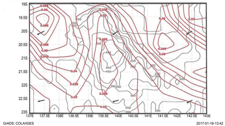
Figure 1. The distribution of the AOD and the topography around the following topographical obstacles: (a) Chibas Mountains (AOD interval of 0.05, topography interval 200 m); (b) Ahagar Mountains (0.03 & 200 m); (c) Gebel Mara (0.03 & 200); (d) Assir Mountains (0.05 & 300); (e) Australia North-West Territories (0.005 & 50).
