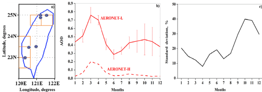
Figure 1. a - the Taiwan area, where the closed circles show the location of AERONET sites, while the orange open boxes represent GEOS-5 model grid boxes located in the vicinity of AERONET sites. Each GEOS-5 model grid box is 0.5^\circ latitude by 0.625^\circ longitude; b - month to month changes in 15-year mean AERONET AOD (2002 – 2017). AERONET-L designates AERONET AOD averaged over the five low-elevated AERONET sites, while AERONET-H designates AOD from the high-elevated (2800 m a.s.l.) Lulin site. The AOD standard deviation is shown by the vertical red lines; c - month to month changes in the AERONET AOD standard deviation from the five low-elevated sites, in percentage to the 15-year mean AOD. (Updated from Kishcha et al. (2018)).
