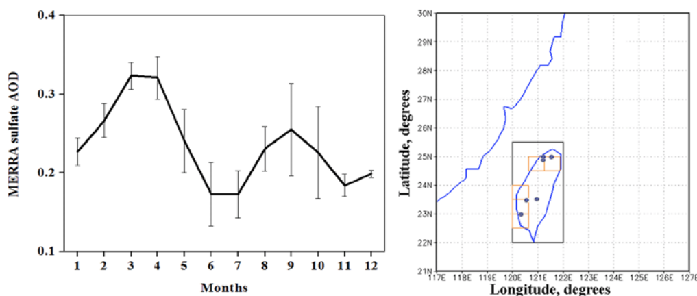
Figure 3. The left panel shows month to month changes in 15-year mean MERRA sulfate AOD over Taiwan. MERRA sulfate AOD was averaged for the five specified GEOS-5 grid boxes of 0.5^\circ latitude by 0.625^\circ longitude each, located in the vicinity of AERONET sites (the orange open boxes on the right panel). The standard deviation of AOD is shown by the black vertical lines. The right panel represents the study area. (Updated from Kishcha et al. (2018)).
