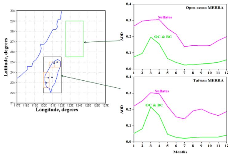
Figure 2. Month to month changes in MERRA AOD over Taiwan and over the open sea area (the green open rectangle in the left panel) in the vicinity of Taiwan, over the 15-year period from 2002 – 2017. The green lines designate organic and black carbon (OC & BC), while the magenta lines designate sulfate aerosols. (Updated from Kishcha et al. (2018)).
