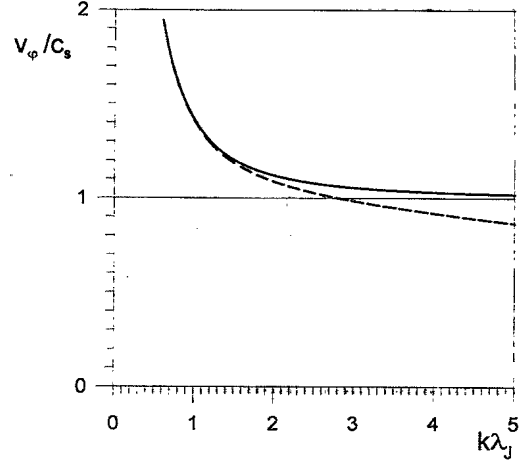
FIG. 2. The dependence of the phase velocity v_\varphi on the wave vector k . The solid line represents a plot using Eq. (8); the dashed line represents a plot using Eq. (11).
