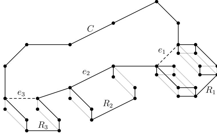
Figure 1: Illustration of the proof of Lemma 3.2. Here, k_1 = 3 and k_2 = 2 . Edges in the cubes R_1 , R_2 and R_3 missing from Q_p^d are depicted in light grey. We fail to extend the cycle C in R_2 : indeed, the right part of R_2 does not contain a maximal monotone path after percolation. However, we manage to replace the (dashed) edges e_1 and e_3 by paths of length 2k_1 + 1 and 2k_2 + 1 in (R_1)_p and (R_3)_p , respectively.
