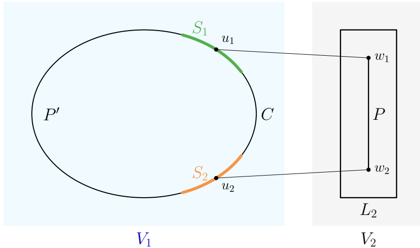
Figure 2: The construction of the cycle C' using the paths P' \subseteq C , P \subseteq L_2 and the edges u_1 w_1, u_2 w_2 connecting the endpoints of P' and P .
