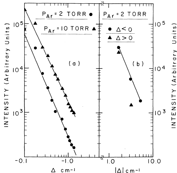
FIG. 2. The dependence of the total re-emitted light intensity, F , on the detuning energy \Delta . \lambda_M = 5688.5 \text{ \AA} , \rho = 9 \text{ cm}^{-1} , p_{Na} = 10^{-1} Torr, and p_{Ar} = 2\text{--}10 Torr. (a) For small values of |\Delta| , F obeys the relation F \propto |\Delta|^{-2.0 \pm 0.2} . (b) For larger values of |\Delta| , this relation holds only for \Delta < 0 while significant deviations from this relation are exhibited for \Delta > 0 .
