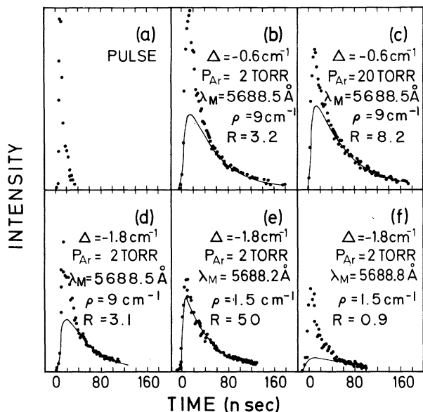
FIG. 1. Time-resolved spectra of the 4^2D_{3/2,5/2} \rightarrow 3^2P_{3/2} transition in Na. \lambda_M is the monochromator wavelength, \rho is the spectral resolution (full width at half-maximum), \Delta is the detuning energy, and R is the ratio of the slow to the fast components. In (b)–(d) \rho \gg \Delta , so that both the resonance fluorescence (RF) and the Raman scattering (RS) components were monitored. In (e) and (f), \rho \lesssim \Delta and the monochromator was set at the central wavelength of the RF component (e) and of the RS component (f). The residual slow component in (f) and the fast component in (e) result from insufficient spectral resolution. The dots represent experimental data, while the solid lines represent the fit for the slow component.
