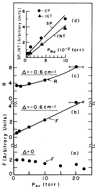
FIG. 3. (a), (b) Dependence of total re-emitted intensity ( F ) on Ar pressure for p_{Na} = 0.1 Torr and (a) \Delta = 0 and (b) \Delta = -0.6 \text{ cm}^{-1} . (c) Dependence of R on p_{Ar} for p_{Na} = 0.1 Torr and \Delta = -0.6 \text{ cm}^{-1} . (d) Dependence on sodium pressure of the intercept (INT) and of the slope (SP) of F vs p_{Ar} plots.
