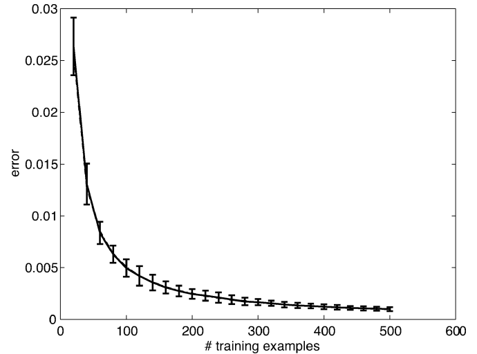
Fig. 6. Error of reconstructing the bias as function of the number of training examples. Here it is assumed that the synaptic matrix is known. Shown are averages and standard deviations of 10 teacher-student experiments.
