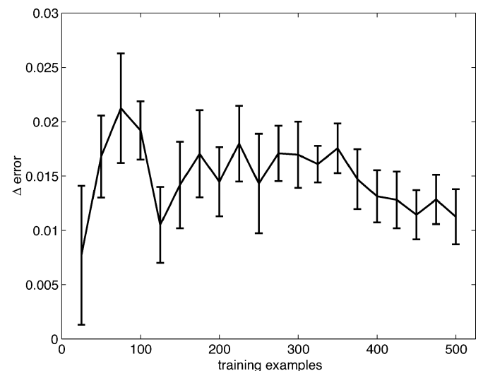
Fig. 7. Difference between errors in networks trained on sequences and those trained on random one-step trials shows the advantage of the latter scheme.
