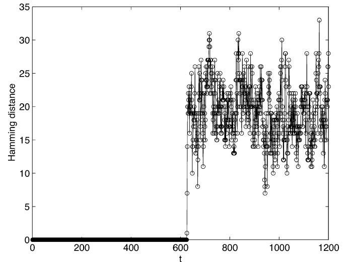
Fig. 2. Hamming distance between two N = 40 spatio-temporal sequences, generated by sets of b_i values that were identical but for a slight change in one of them.
