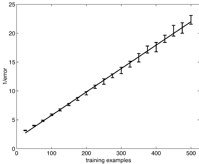
Fig. 5. Inverse error is proportional to the number of training examples, as shown here for the averages of 10 teacher-student experiments.
