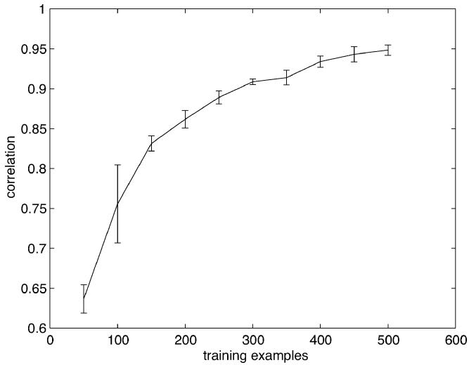
Fig. 3. Correlation between teacher and student DNF in the N = 40 problem, using the perceptron algorithm in 10 different teacher-student experiments.
