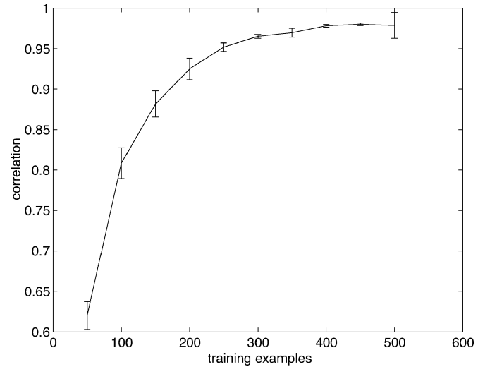
Fig. 8. Correlation between teacher and student DNF using the SVM learning algorithm. The error bars represent standard deviations of 10 different teacher-student experiments.
