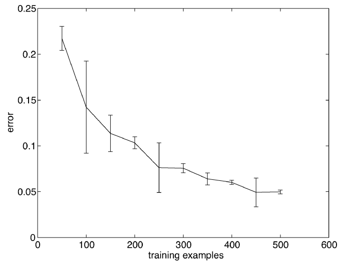
Fig. 4. Convergence of the errors of student networks on one-step prediction tasks.
