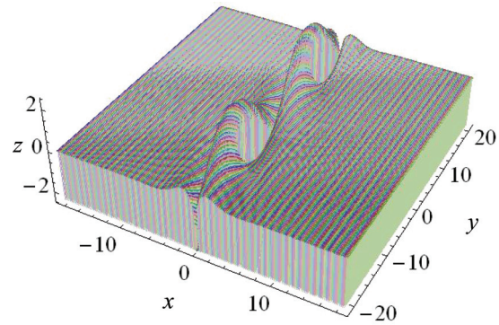
FIG. 3. (Color online) Shape of a folded sheet whose y invariance is broken by a “soft v mode.” Vertical scale is expanded for clarity. Colored stripes are planes of constant u . Dots are spaced equally in the material, so that the variable spacing between them indicates strain. Near edges at y = \pm 20 are symmetric folds pointed downward; two symmetric folds pointed upward appear as peaks. Each xz cut is one of the degenerate solutions given by Eq. (10) with c_2 = 0 and c_1 that changes linearly with y . The pressure is P = 0.5 .
