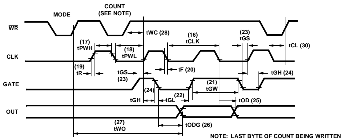
FIGURE 20. CLOCK AND GATE
