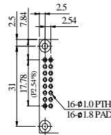
PIN DETAIL
