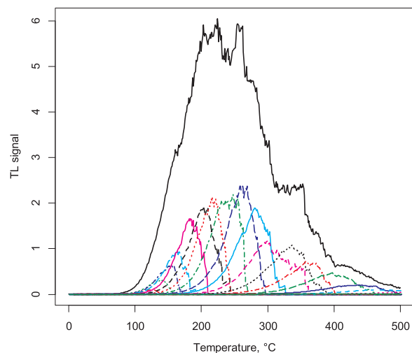
Fig. 7. Example of the output from the MC procedure for a TL glow curve, showing how the broad TL glow curves in feldspars can be considered as a sum of several first-order TL glow peaks with a distribution of amplitudes given by the symmetric function shown in Eq. (7).
