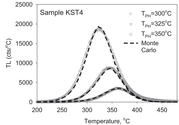
Fig. 5. The TL glow curves for a second set of measurements with a fixed preheat time t_{PH} = 10 \text{ s} and a variable preheat temperature T_{PH} = 300, 325, 350 \text{ }^\circ\text{C} . The MC simulation are shown as dashed lines, and the critical distances are: r'_c = 0.85, 1.13, 1.3 . The rest of the fitting parameters are the same as in Fig. 4.
