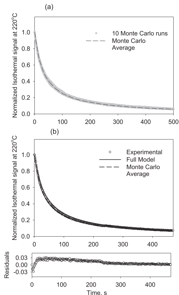
Fig. 2. (a) MC simulation of an isothermal experiment for irradiated Durango apatite. The temperature is raised to 220^\circ\text{C} and kept constant for 500 s (Sfampa et al., [5]). The parameters in the MC simulation are \rho' = 0.007 , A_{ISOTH} = 0.20 \text{ s}^{-1} . The gray area in (a) indicates the overall results from 10 MC simulations of 200 electrons each, and the dashed line indicates the average of these 10 runs. (b) The experimental data (open circles) are compared with the MC simulation (dashed line), and with the exact solution obtained by the numerical integration of Eq. (3) (solid line). The fitting residuals shown are of the order of 3% or better.
