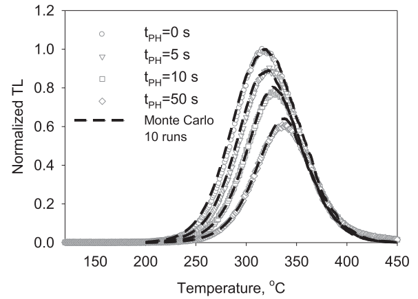
Fig. 4. The irradiated microcline KST4 sample was preheated to T_{PH} = 300 \text{ }^\circ\text{C} and this preheat temperature was held fixed for a variable preheat time t_{PH} = 0, 5, 10, 50 \text{ s} . It is assumed that these preheated samples can be described using a truncated distribution function, and the critical radius is treated as an adjustable fitting parameter. The MC results are shown as dashed lines, and the fitting parameters are: E = 1.45 \text{ eV}, A_{TL} = 3.5 \times 10^{12} \text{ s}^{-1} , and r'_c = 0, 0.7, 0.77, 0.86 .
