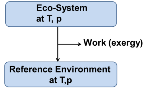
Figure 4. Eco-exergy definition
