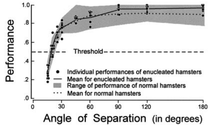
FIG. 16. Sound localization performance of normal (shading) and blind (filled circles) hamsters for a single 100-ms noise burst. Average performance for 12 normal and eight blind hamsters is indicated by a broken and a solid line, respectively. There was no difference in threshold between the two groups. The apparent superiority of the blind hamsters at large angles is significant only at 120 and 180°.
