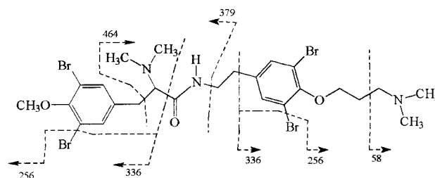
Figure 1. EIMS fragmentation of 1 .
