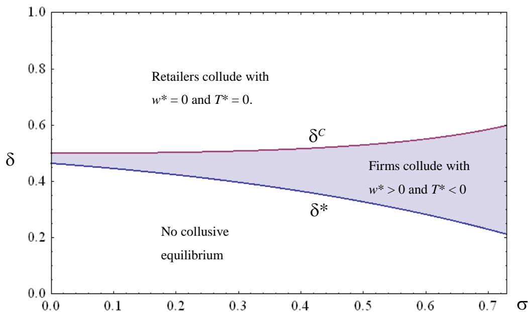
Figure 2: The cutoffs \delta^C and \delta^* as a function of \sigma
