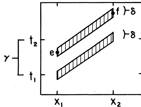
FIG. 6. A measurement of J_x is carried out at (x_1, t_1) and (x_2, t_2) and a measurement of J_y is carried out at e and f . The two measurements will not disrupt one another and the original state |\alpha\rangle_- will be restored at the end of the process.
