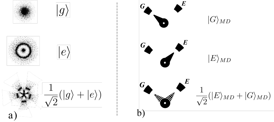
Figure 1: Superposition principle. a) If an atom can be in state |g\rangle and it can be in state |e\rangle then it can be in state \frac{1}{\sqrt{2}}(|g\rangle + |e\rangle) . b) If a pointer of the measuring device can be in state |G\rangle_{MD} and it can be in state |E\rangle_{MD} then it can be in state \frac{1}{\sqrt{2}}(|G\rangle_{MD} + |E\rangle_{MD}) . For macroscopic measuring devices the principle holds in the the framework of MWI, but it does not hold in the frameworks of single-world interpretations.
