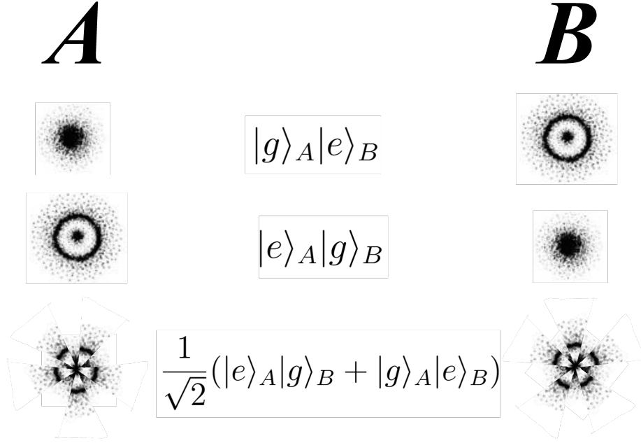
Figure 2: Separated atoms in an entangled state. The superposition principle holds for separated atoms. We have two different states in which one atom is in the ground state and another in excited state. The superposition of these states exists too.
