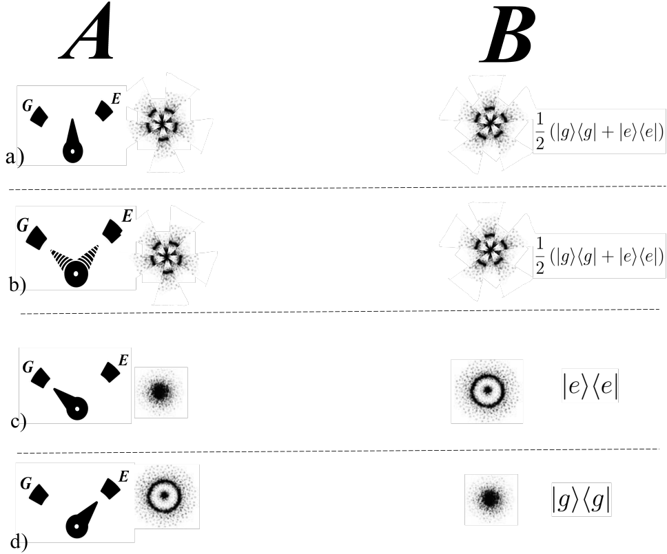
Figure 3: Action at a distance. a) Description of entangled atoms before a measurement in A . b) Description of entangled atoms after a measurement in A in the framework of MWI. Local description in B remains the same as it was in (a). c-d) Description of entangled atoms after a measurement in A in the framework of single-world interpretations. There are two possible different outcomes, but in both cases the local description in B is different from what it was in (a).
