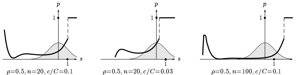
Figure 1: Equilibrium participation probability function computed numerically
