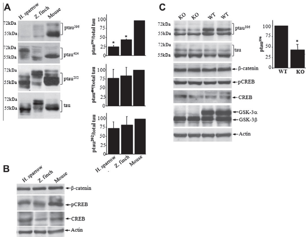
Fig. 2. Lack of GSK-3 \alpha results in reduced tau phosphorylation. (A) Brain tissue extracts (60 \mu g) prepared from house sparrow, zebra finch and mouse were subjected to gel electrophoresis and western blot analysis using the indicated anti-phospho-tau (Ser 396, Ser 404 and Ser 202) antibodies. Densitometry analysis of the phosphorylated fraction of tau (phospho-tau/total tau) is shown in the right panel and is fold of the phosphorylated fraction obtained for mouse tau that was designated to 100%. Results are mean \pm S.E.M. ( n = 3 ). Tau isoforms migrate as proteins ranging from 52 to 72 kDa. (B) The same as A except that anti- \beta -catenin, anti-phospho-CREB (Ser129/133), and anti-CREB antibodies were used. Expression of actin is shown to confirm equal loading. (C) Hippocampus tissue extracts (60 \mu g) prepared from GSK-3 \alpha KO and WT were subjected to western blot analysis using the same antibodies described in (A). Densitometry analysis of phosphorylated tau is shown in the right panel as a mean \pm S.E.M. ( n = 4 ). Gels are representative of three individuals of each species of bird and four KO and four WT mice.
