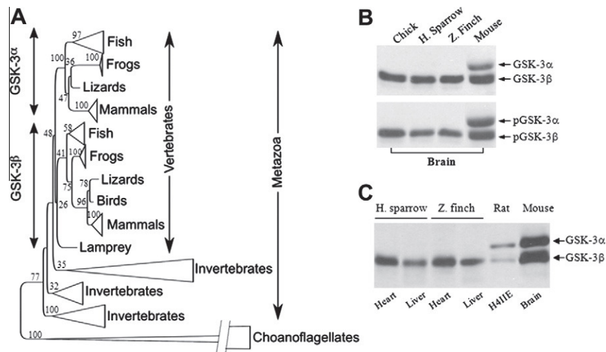
Fig. 1. GSK-3 \alpha is missing in birds. (A) Schematic representation of a phylogenetic tree calculated from multiple sequence alignment of diverse GSK-3 sequences (see Fig. S1 for complete data). Triangles cluster several species of the noted groups. Alpha and Beta labeled arrows show groups where GSK-3 \alpha and GSK-3 \beta sequences, respectively, were found. Note that a GSK-3 gene from a lamprey ( Petromyzon marinus ), a basal jawless vertebrate, was found within the GSK-3 \beta group and that GSK-3 sequences from non-vertebrate basal chordates ( Amphioxus , a cephalochordate, and Saccoglossus , a hemichordate) were placed in groups outside the \alpha and \beta GSK-3 sequences (Fig. S1). The unicellular choanoflagellates (the ancestors of sponges) were used as the out group to root the tree. No GSK-3 \alpha genes were found in birds. Bootstrap values are shown. (B) Expression of GSK-3 proteins in brains of chicken embryo (day 18), house sparrow, zebra finch and mouse. Brain tissue extracts (60 \mu g) were subjected to western blot analysis using anti-GSK-3 (upper panel) or anti-phospho-GSK-3 (Tyr 216/279) (lower panel) antibodies. Shown are representative gels from three independent experiments.
