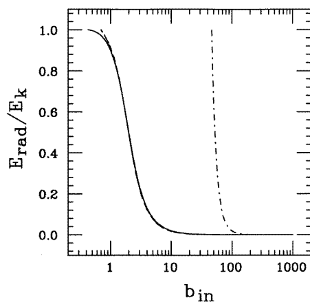
Figure 4. The ratio between the entire energy radiated and the initial kinetic energy is plotted as a function of the impact parameter of the incoming charge. Each curve denotes a set of solutions as in figure 2.
