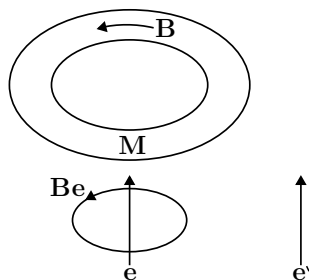
Figure 3: The Tonomura experiment (see text).
