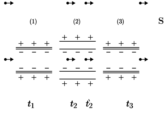
Figure 1: The electric AB effect (see text).
