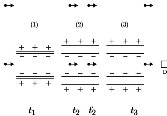
Figure 2: A refutation of the electric AB effect (see text).
