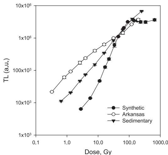
Figure 1. The TL vs. dose-response of the ‘110°C’ glow-peak of the three quartz types as a function of the dose.
