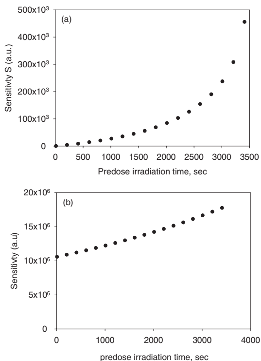
Figure 4. The results of the simulation of the experiments (a) Sensitivity vs. predose only and (b) Sensitivity vs. predose after heating to 500°C. These are to be compared with the experimental data shown in Figures 2 and 3 above.
