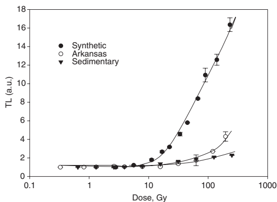
Figure 2. The sensitivity of the ‘110°C’ glow-peak as a function of the predose only, normalised to the sensitivity at the lowest predose.
