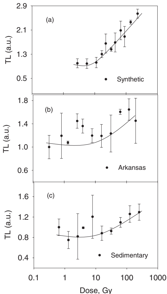
Figure 3. The sensitivity of the '110°C' glow-peak for samples that underwent both a predose irradiation and a thermal activation up to 500°C, normalised to the sensitivity at the lowest predose. (a) synthetic (b) Arkansas (c) sedimentary quartz.
