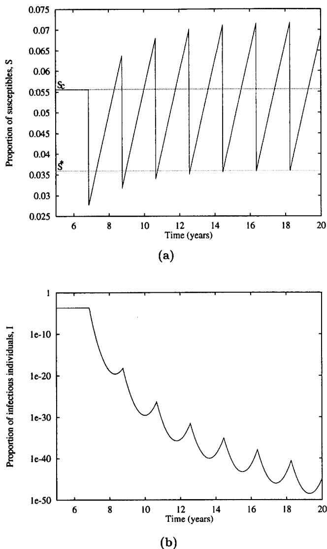
Figure 2. (a) The proportion of susceptibles S when pulse vaccination is applied ( p = 0.5 , and T = 2 ) to the SIR model (1). The susceptibles are attracted to a periodic “infection-free” solution (16). The line at S_c \approx 0.0556 marks the “epidemic threshold” (22). (b) Time-series for the corresponding rapidly decreasing infectious population I . Note the logarithmic scale employed. Model parameters as given in (3).
